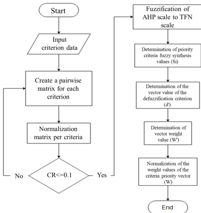
Fig. 2. Fuzzy AHP process for ranking
